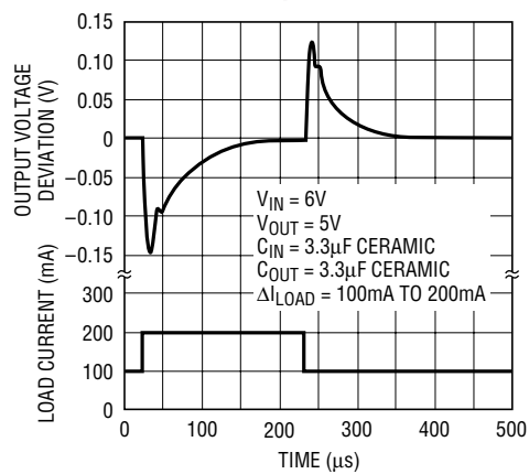
Transient Response
